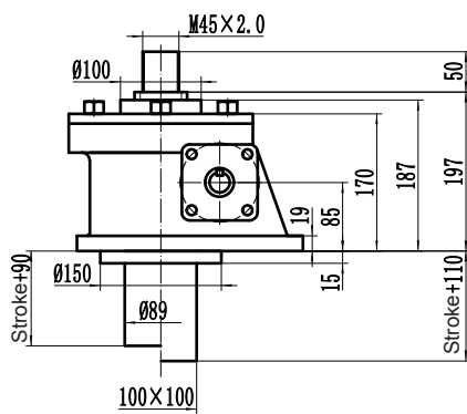
US, UK : Upright translating screw( Screw anti-rotation )
