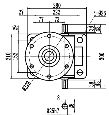
Mounting View
