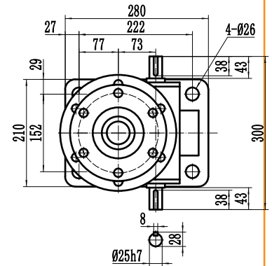
Mounting View
