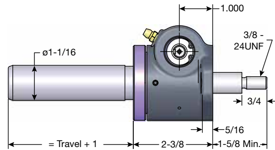
Inverted: B9250TV
