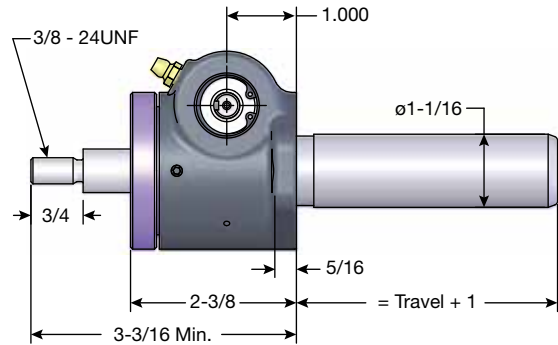
Upright: B9250T
