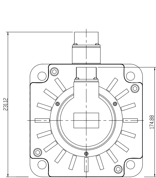
DIMENSION TABLE (MODEL WITHOUT BRAKE)
