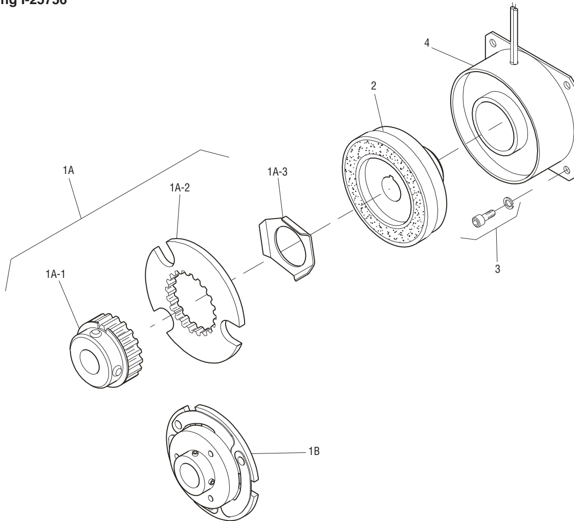
Drawing I-25756
