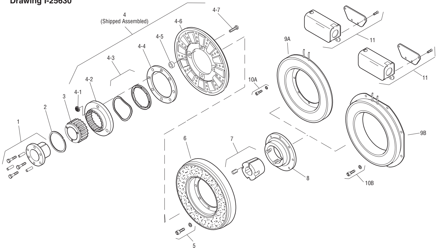
Drawing I-25630
