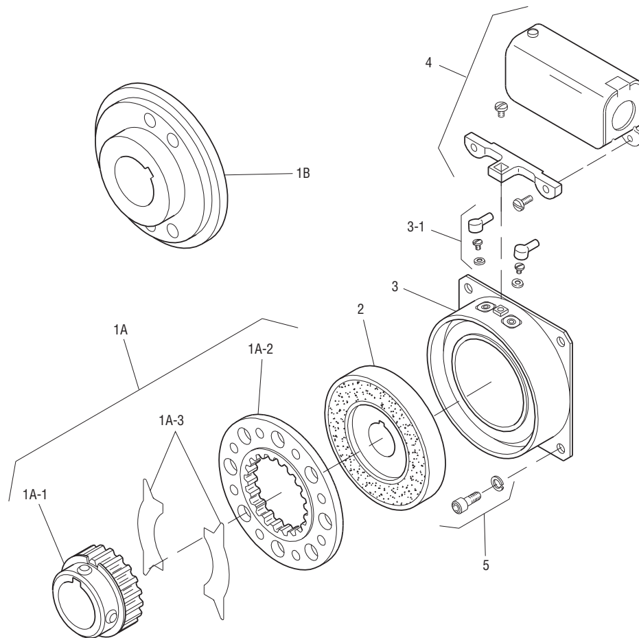
Drawing I-25697
