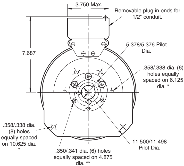
FIELD VIEW
