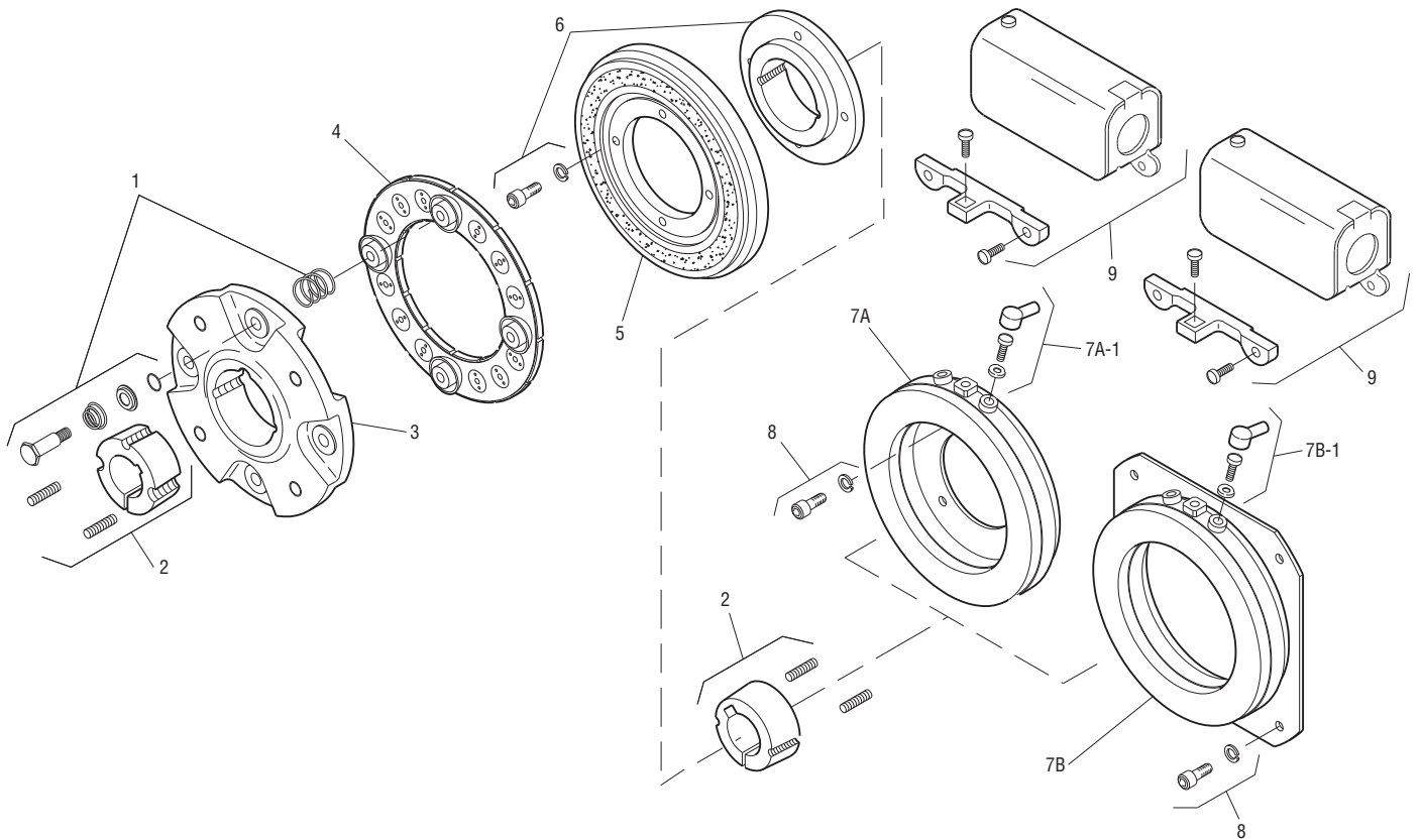
Drawing I-25728
