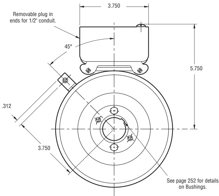
FIELD VIEW
