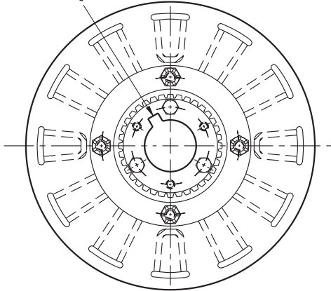
ARMATURE VIEW
