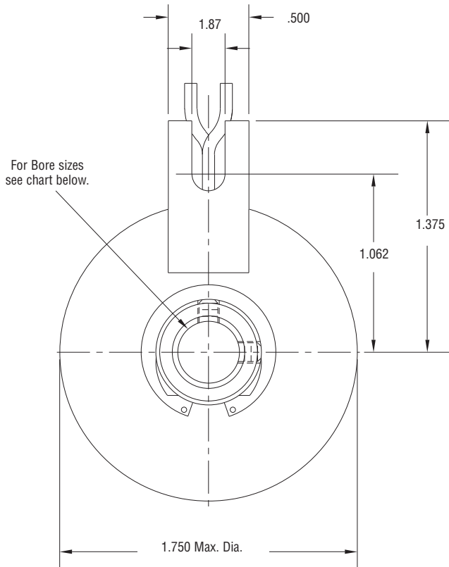
FIELD VIEW
