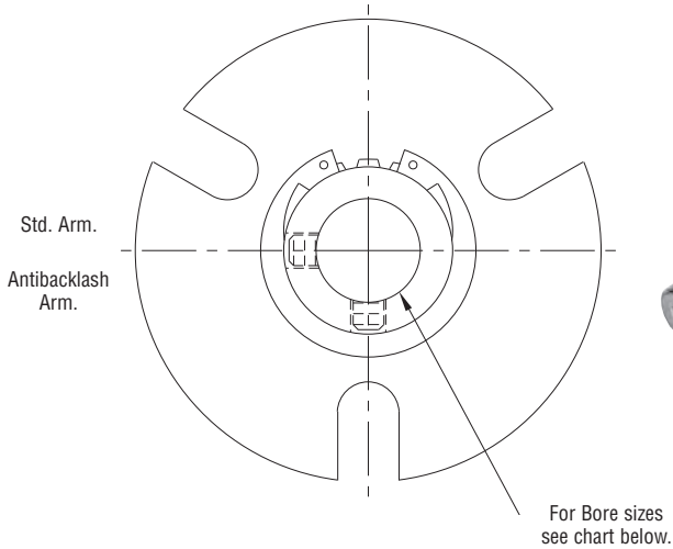
ARMATURE VIEW
