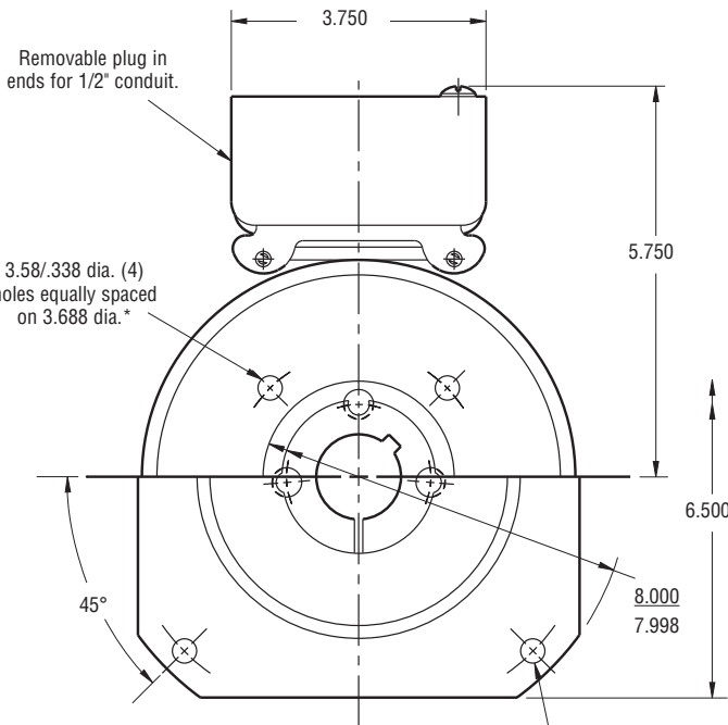
HUB VIEW
