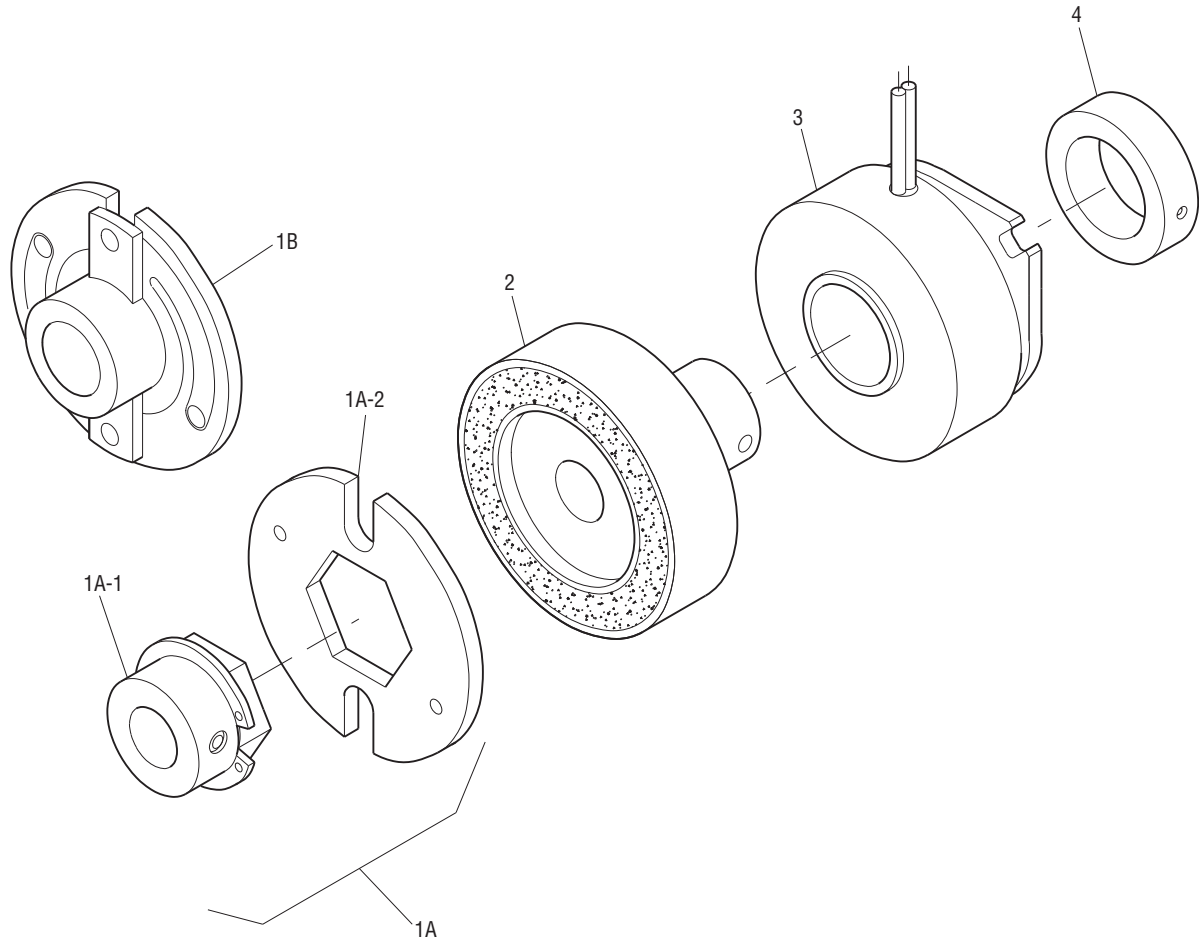
Drawing I-25504
