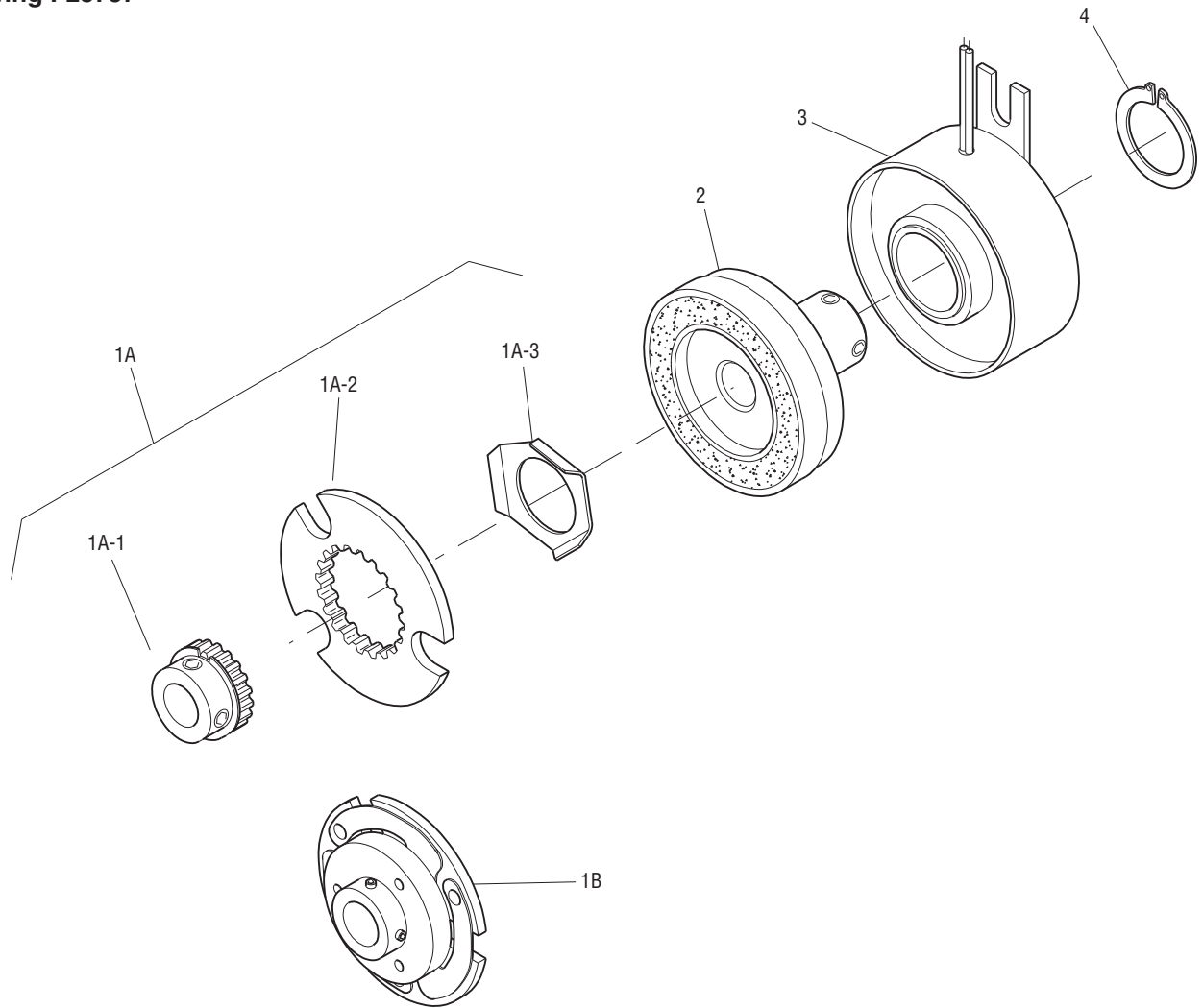
Drawing I-25757
