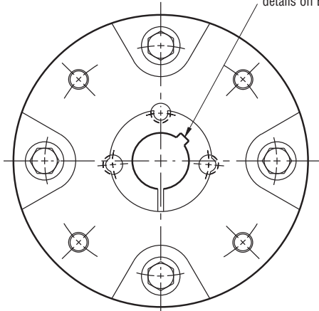
HUB VIEW
