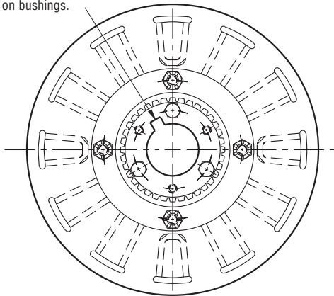
ARMATURE VIEW
