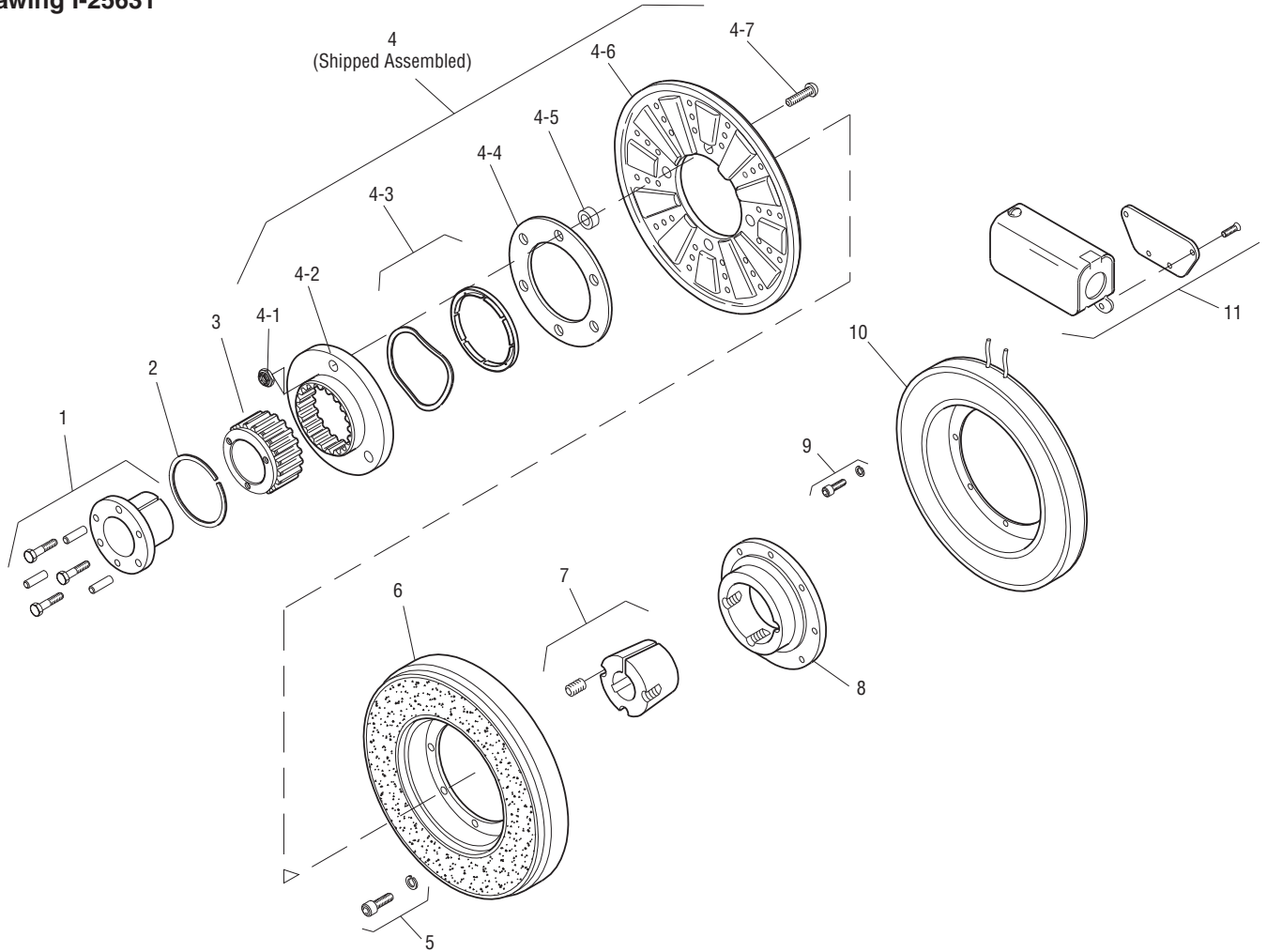
Drawing I-25631
