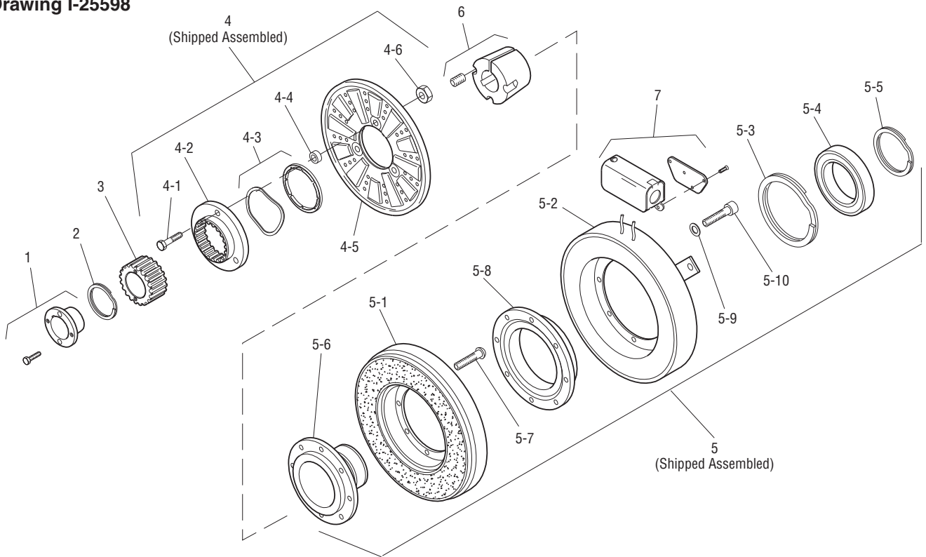
Drawing I-25598
