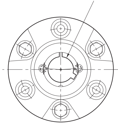
HUB VIEW
