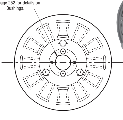
ARMATURE VIEW
