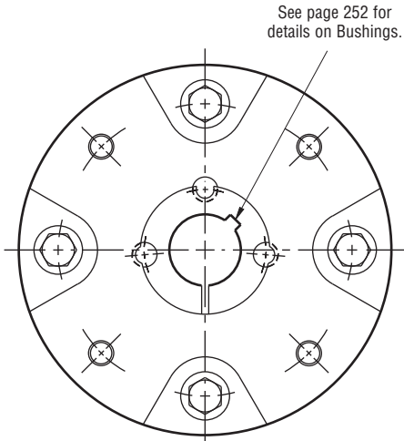
HUB VIEW
