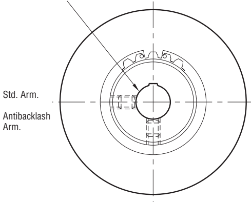
ARMATURE VIEW
