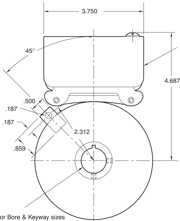
FIELD VIEW
