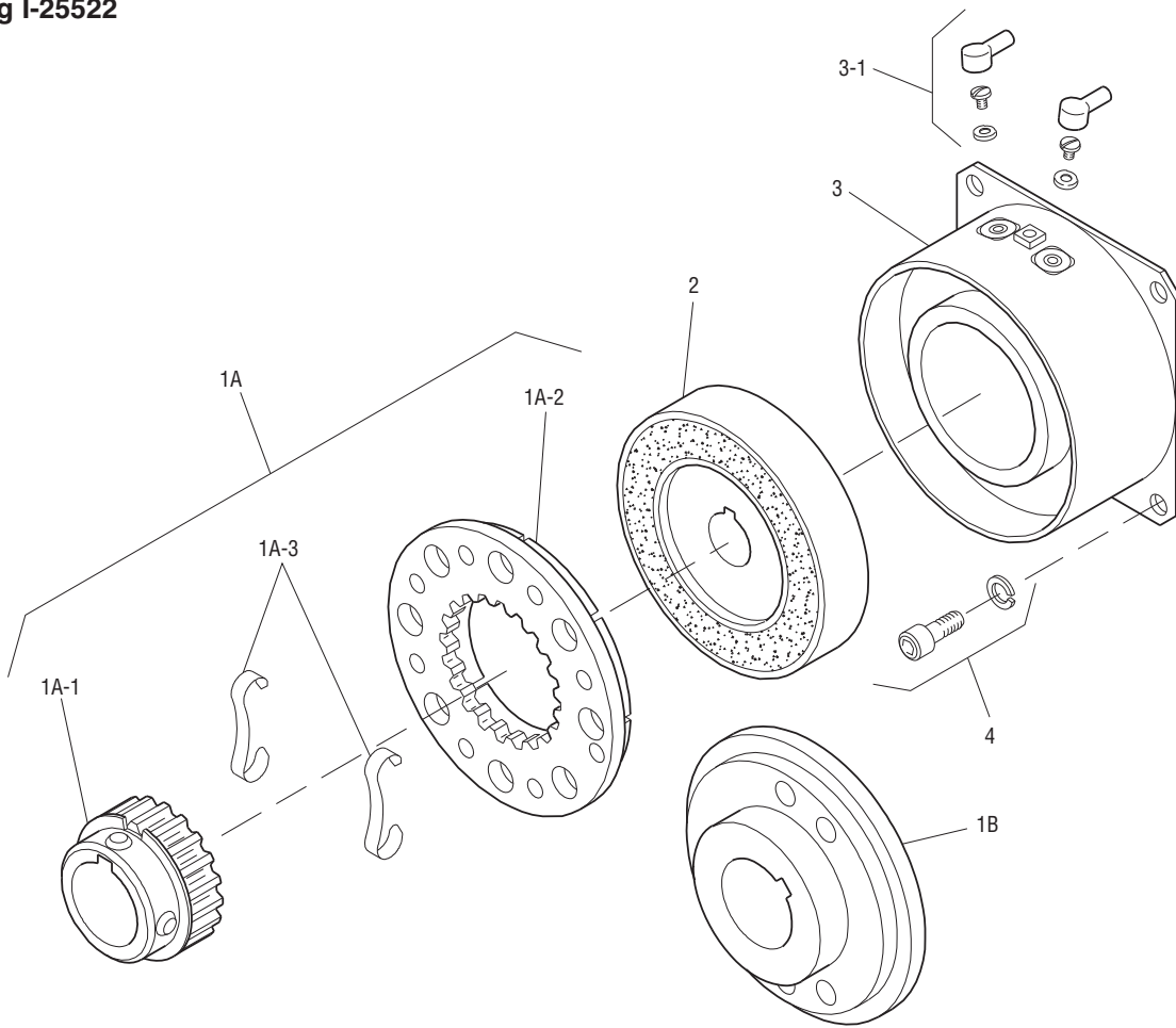
Drawing I-25522
