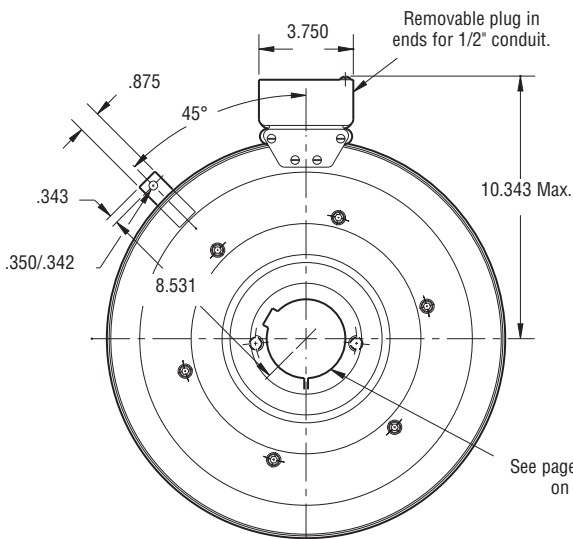
FIELD VIEW
