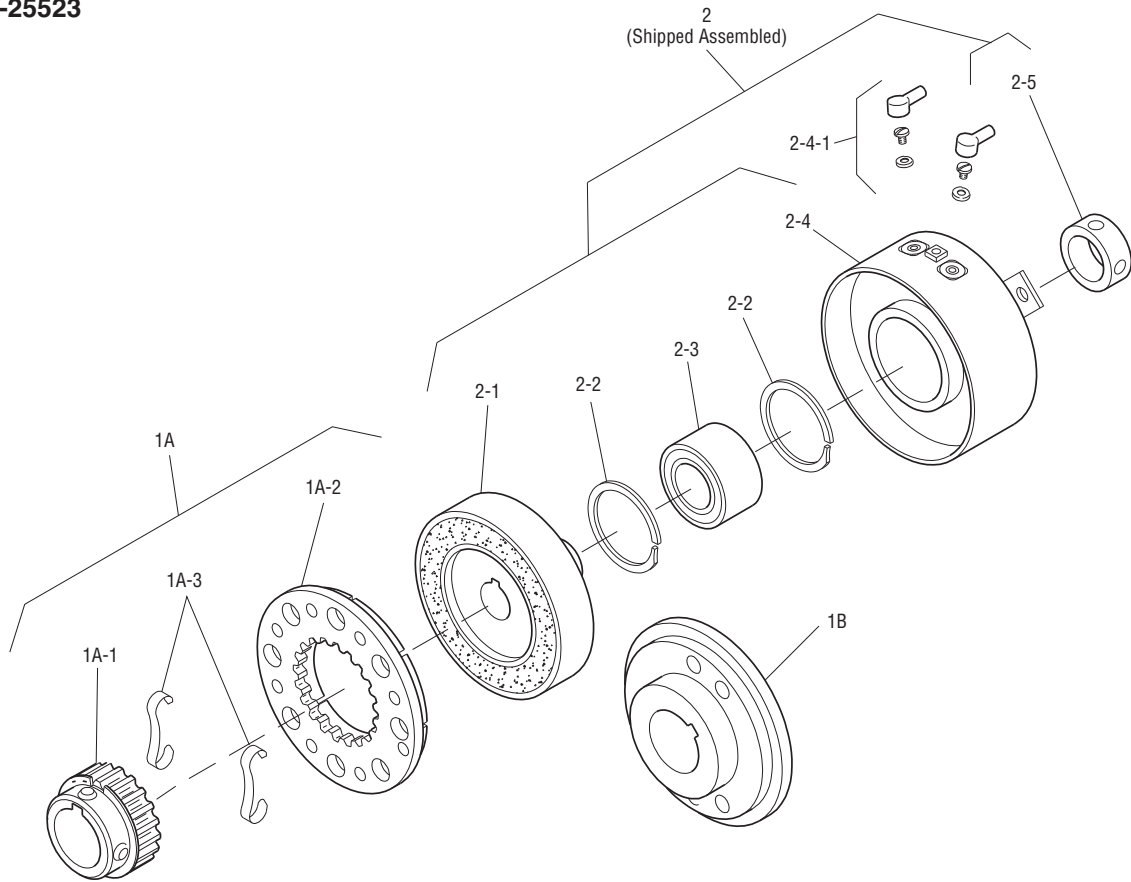
Drawing I-25523
