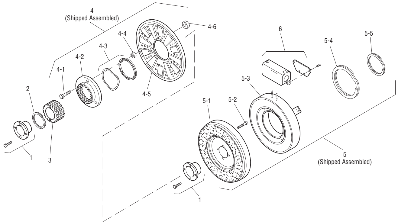
Drawing I-25574
