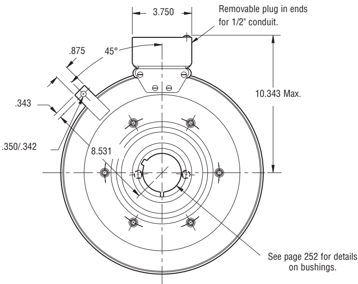
FIELD VIEW
