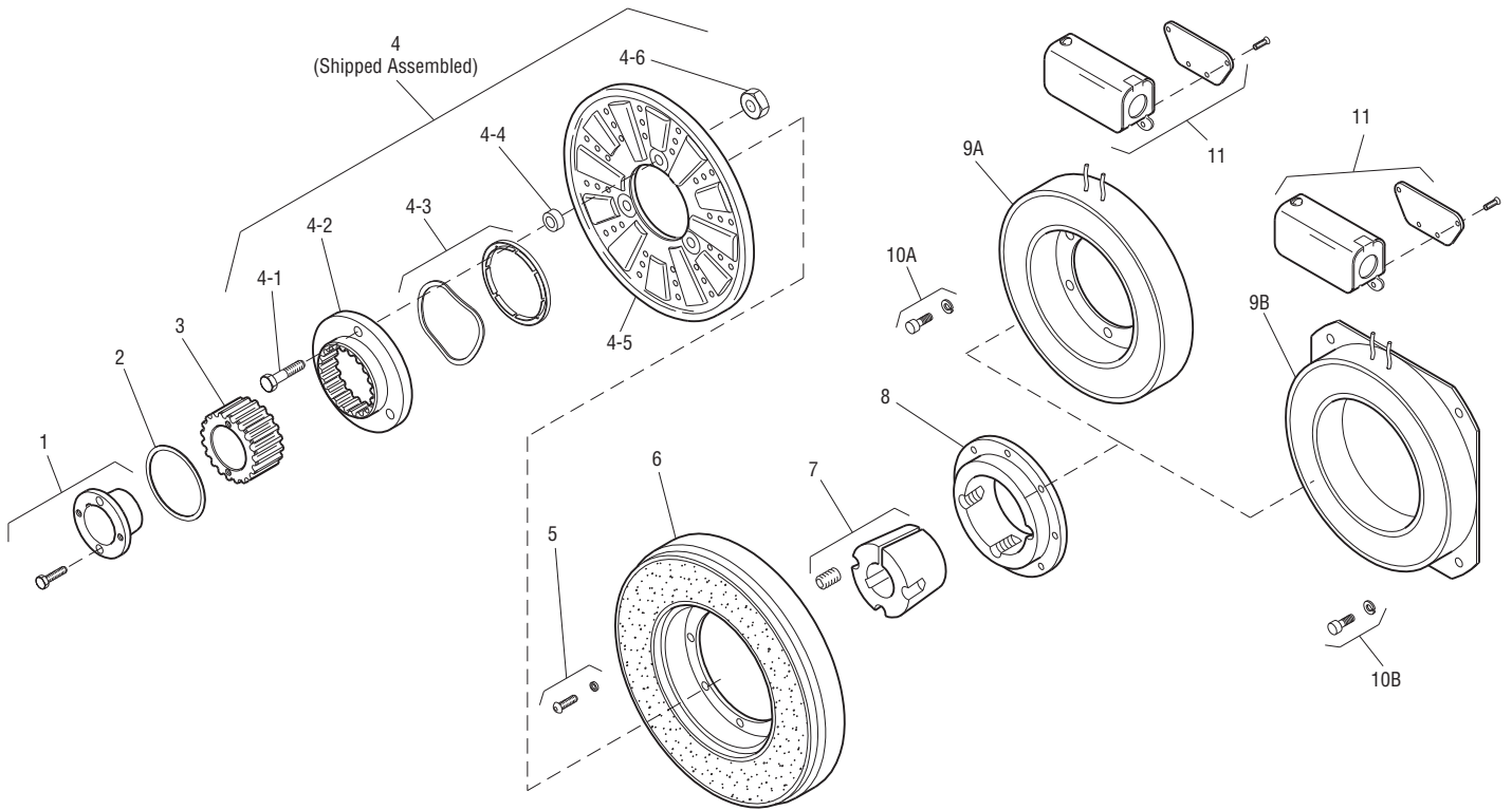
Drawing I-25584
