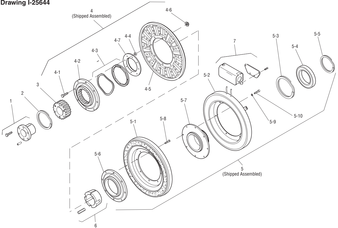
Drawing I-25644
