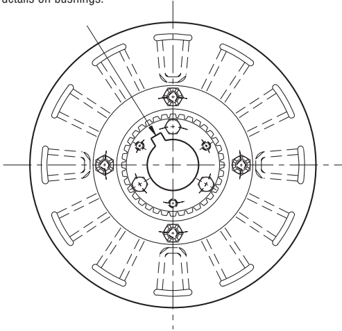
ARMATURE VIEW
