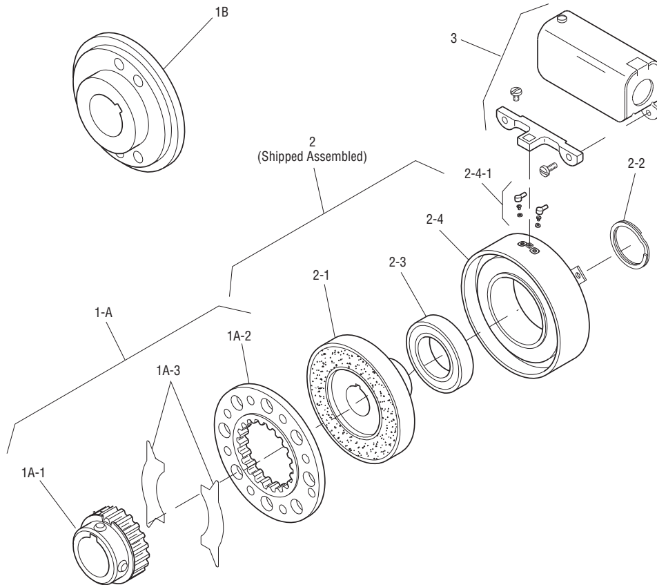
Drawing I-25698
