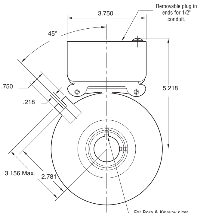
FIELD VIEW
