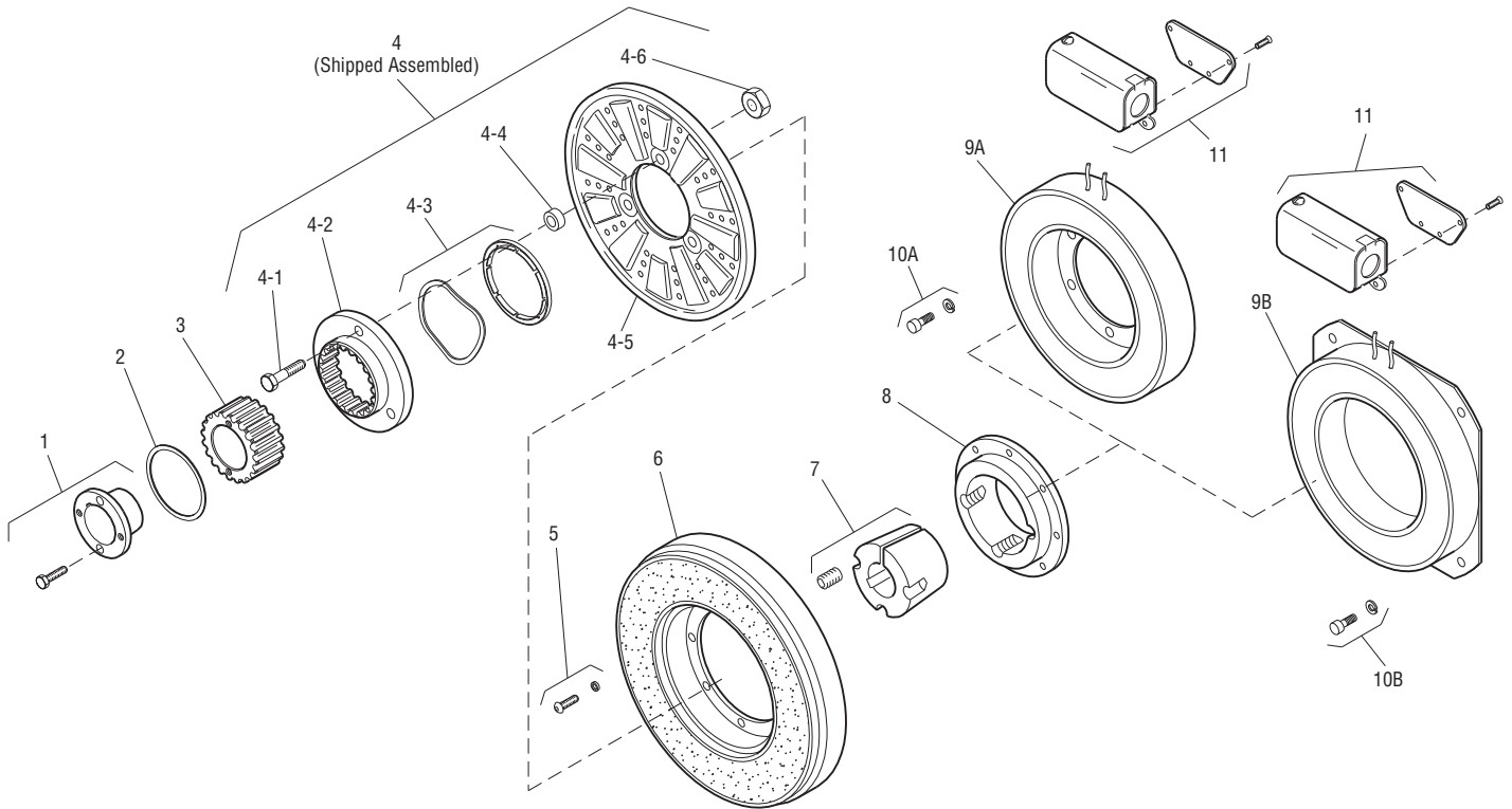
Drawing I-25564
