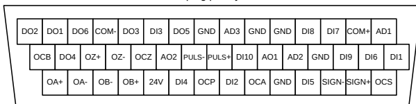
CN1 plug signal layout
